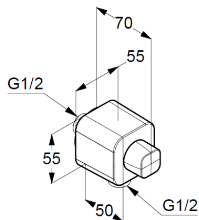
Dimensional drawing
