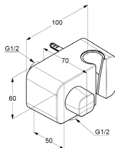
Dimensional drawing
