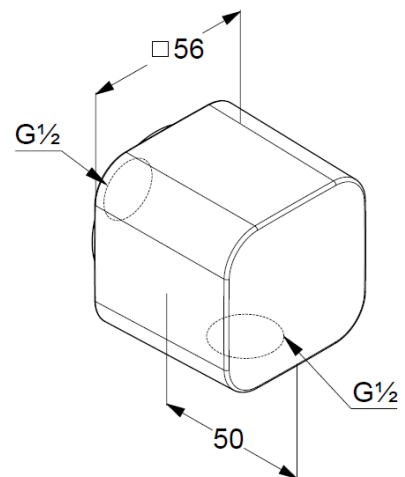
Dimensional drawing
