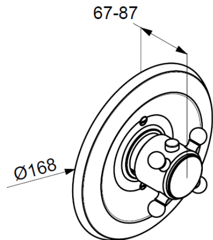
Dimensional drawing
